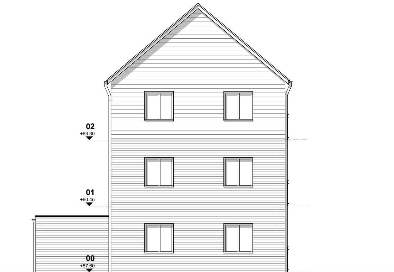
West Elevation
