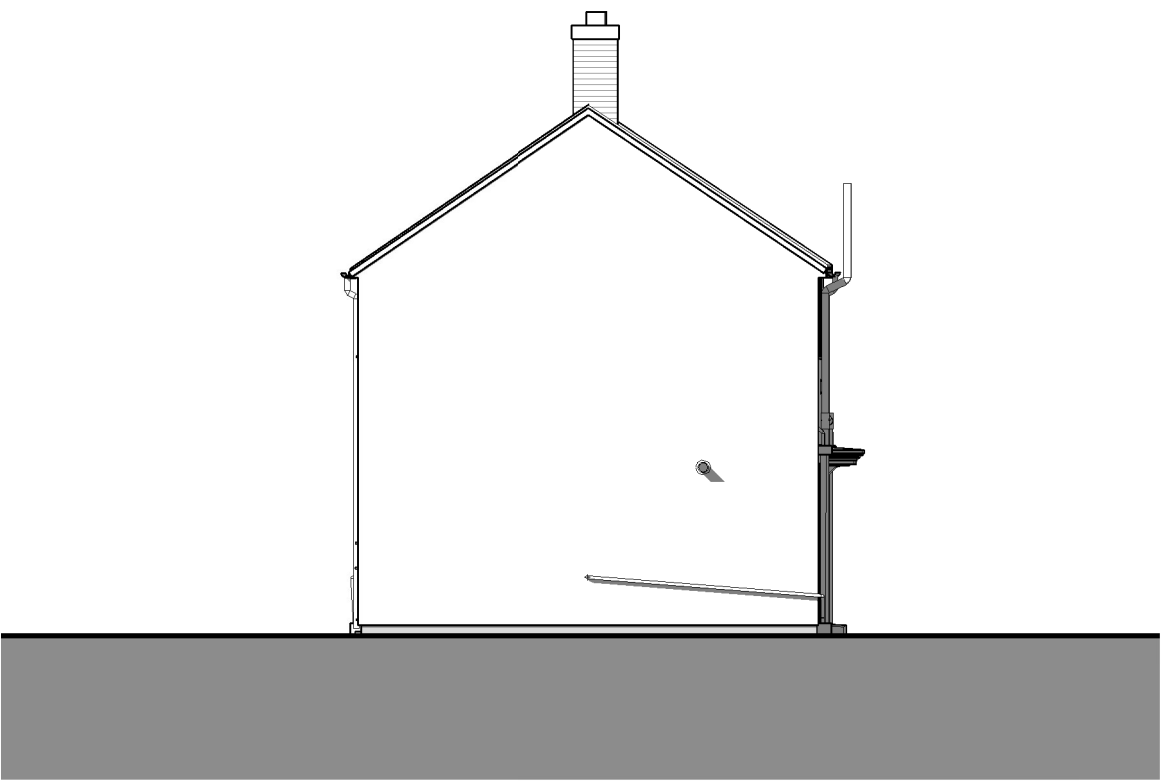
Left Side Elevation as Existing
