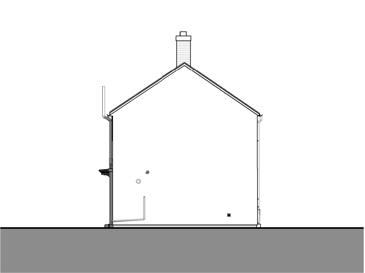
Right Side Elevation as Proposed
