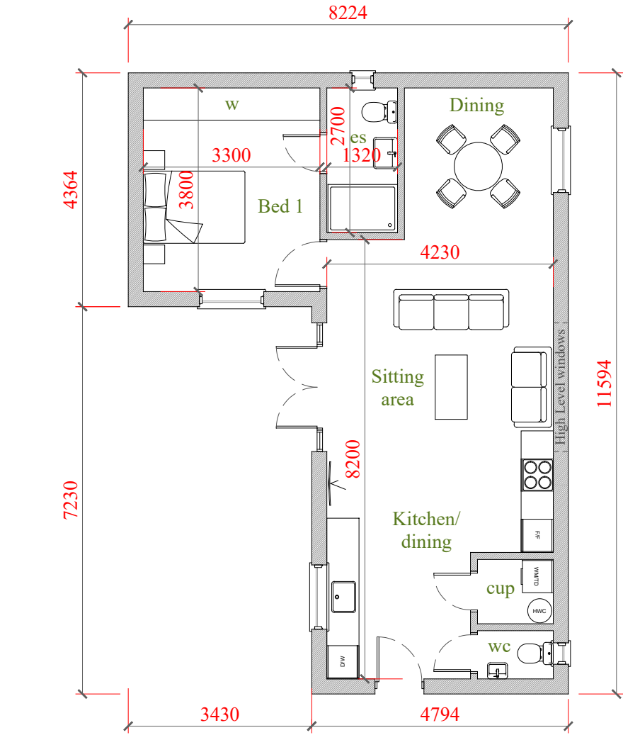
Ground Floor Plan 1:100 PROPOSED
