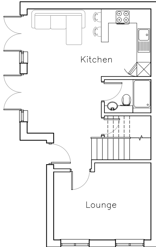
Ground Floor 1:100
