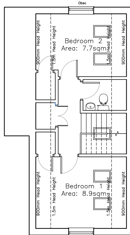
First Floor 1:100
