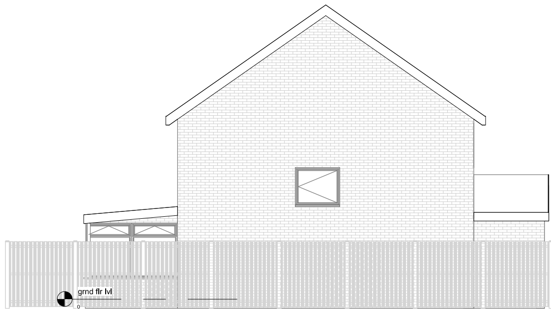
Existing Elevation-Left side
