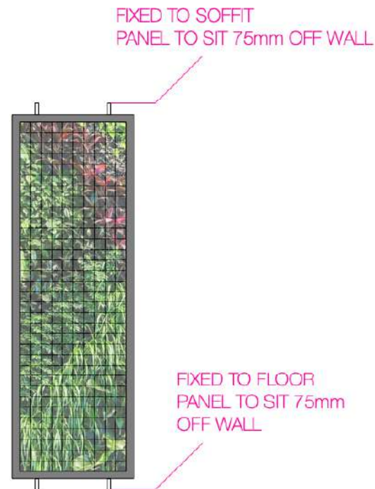
PANEL ELEVATION
