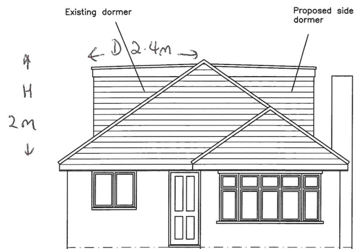
Front Elevation 1:100
