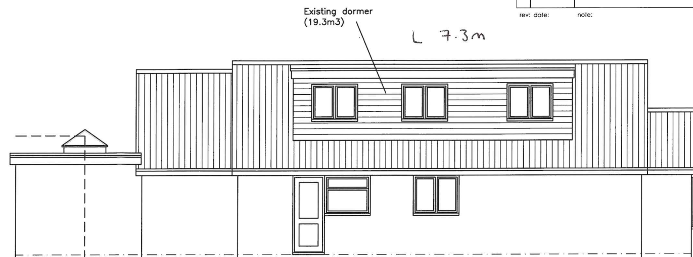
Side Elevation
