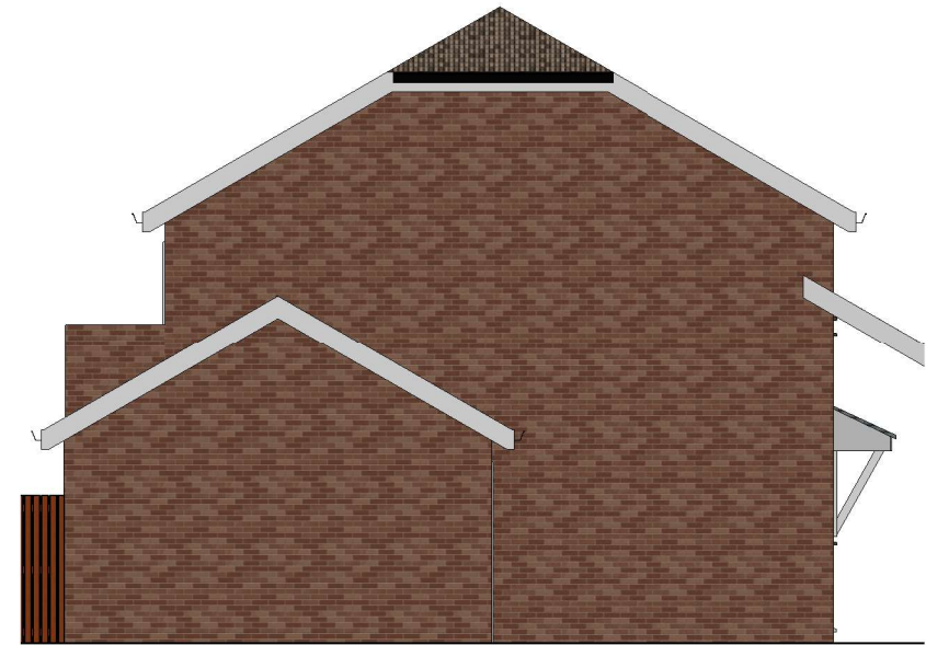
2 North Elevation 1 : 100
