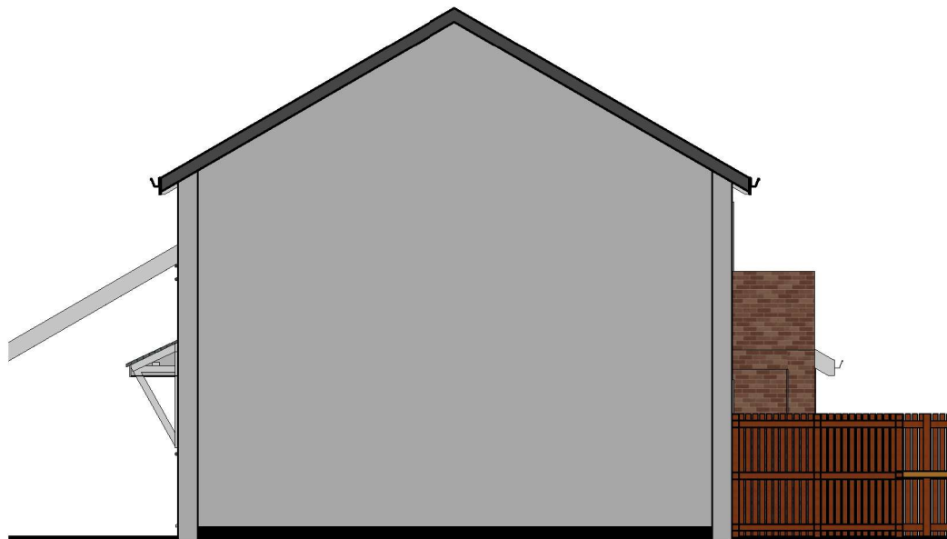
3 South Elevation 1 : 100
