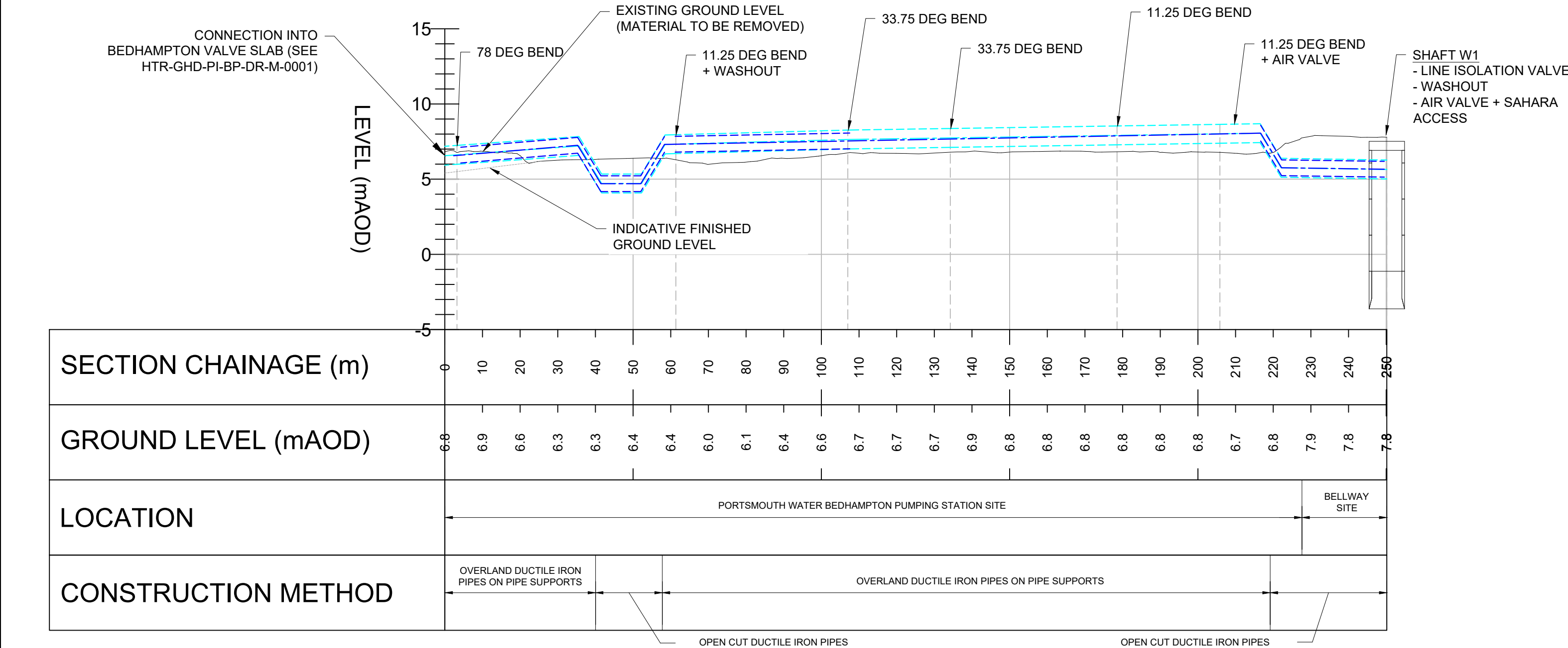
BEDHAMPTON TO HTR DUAL PIPELINES LONGSECTION (H 1:1000, V 1:250)
