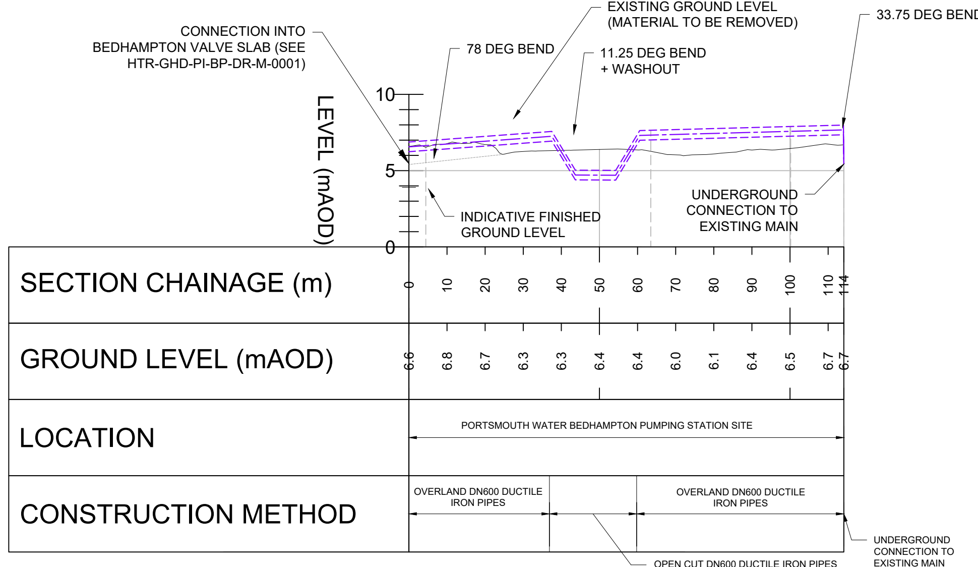
FARLINGTON CONNECTION PIPELINE LONGSECTION (H 1:1000, V 1:250)
