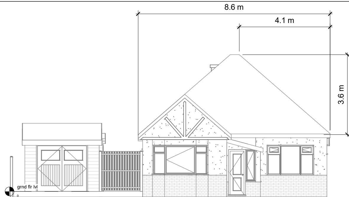
Existing Elevation-Front
