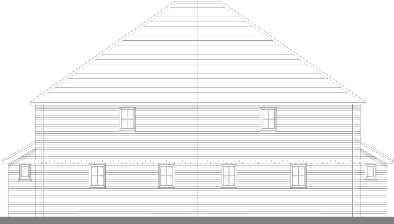
Side Elevation
