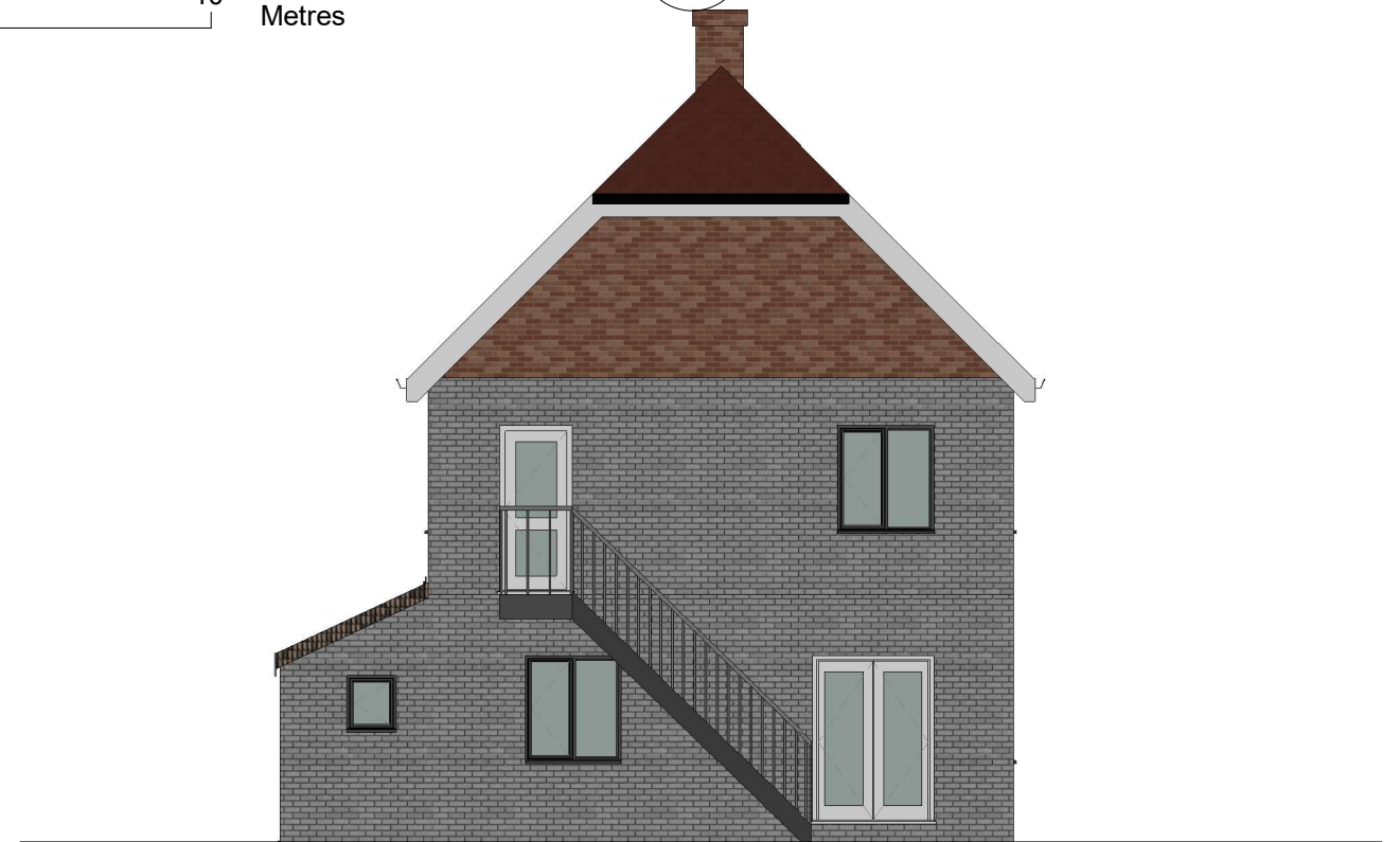
4 West Elevation 1 : 100
