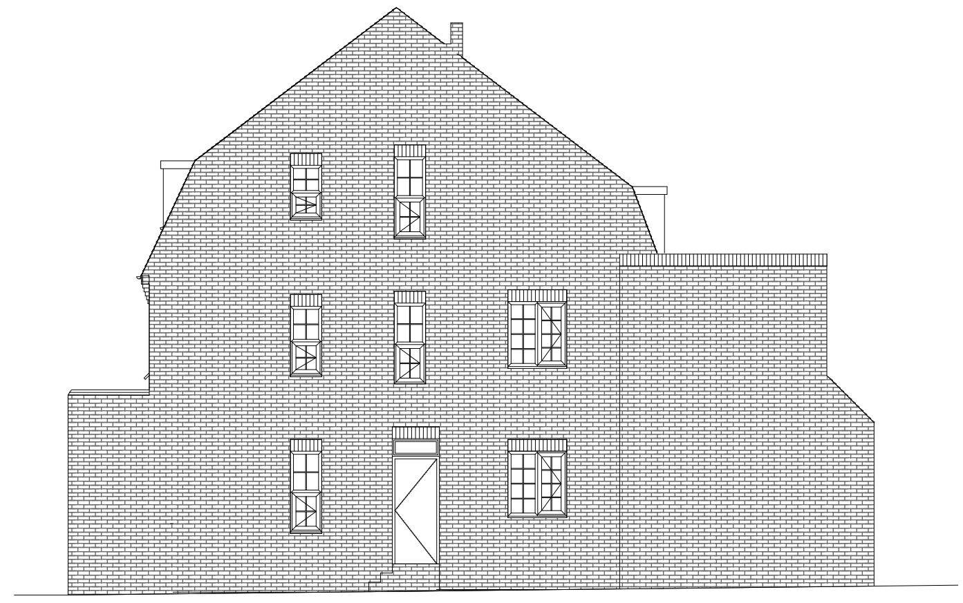
WEST ELEVATION 1:100
