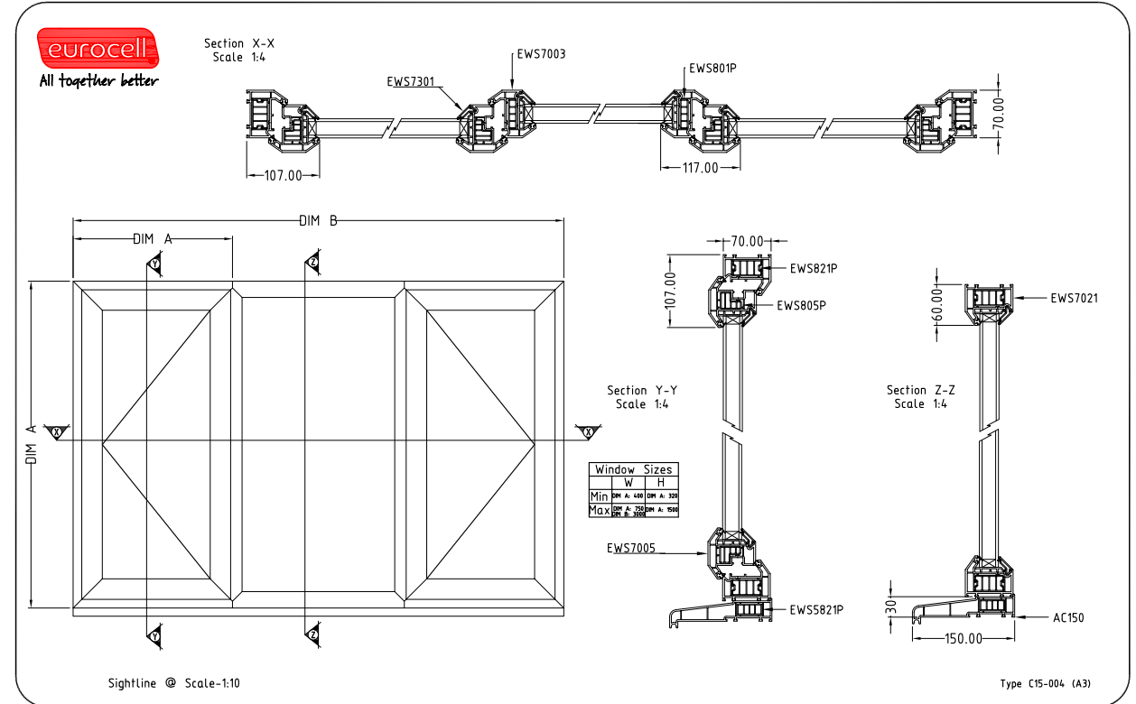
TYPICAL WHITE uPVC WINDOW SECTION NEW WINDOWS 1:10
