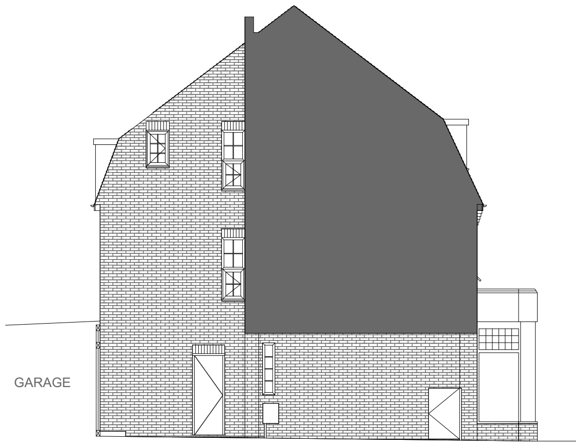
EAST ELEVATION 1:100
