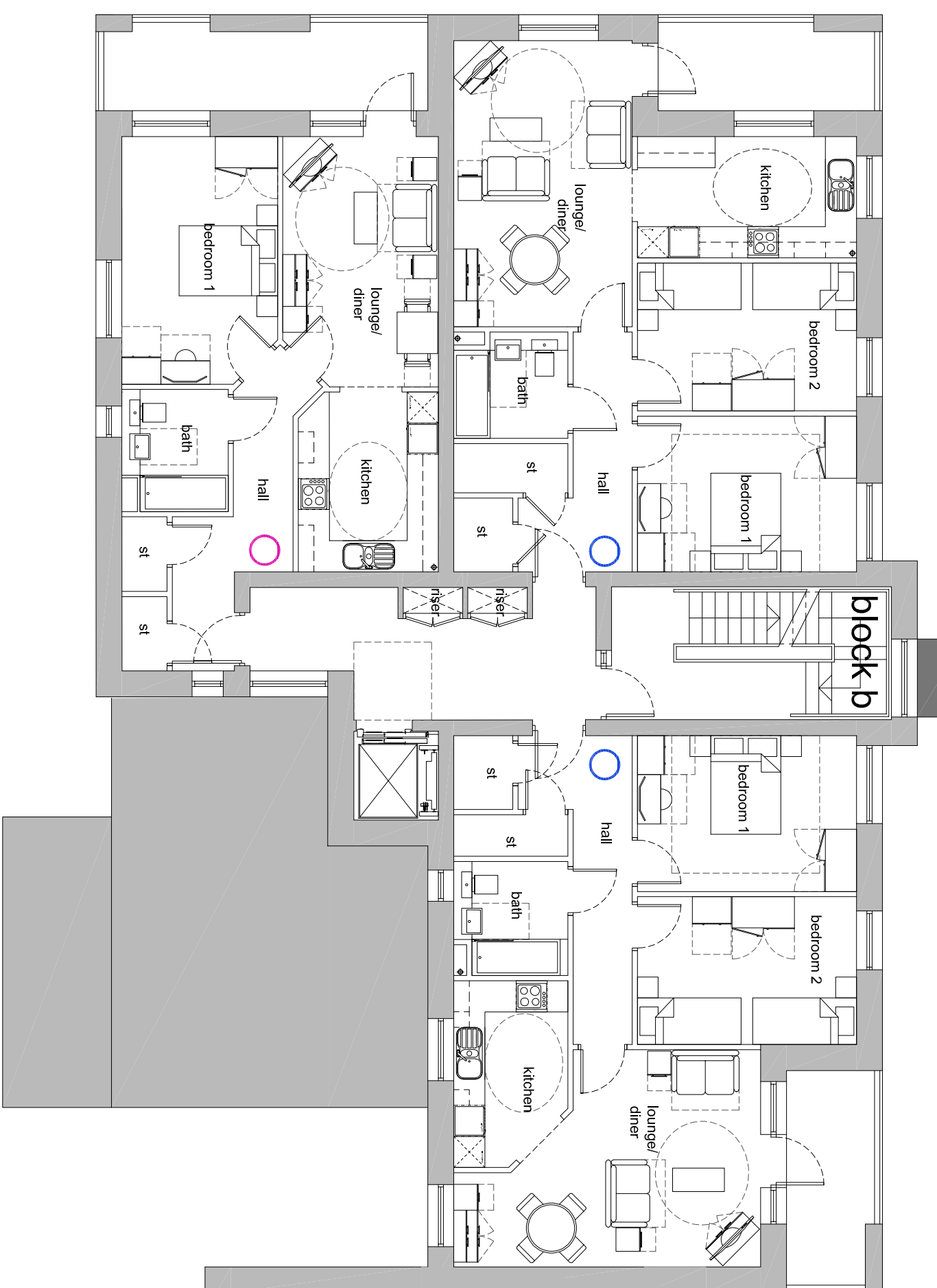
2nd floor plan
