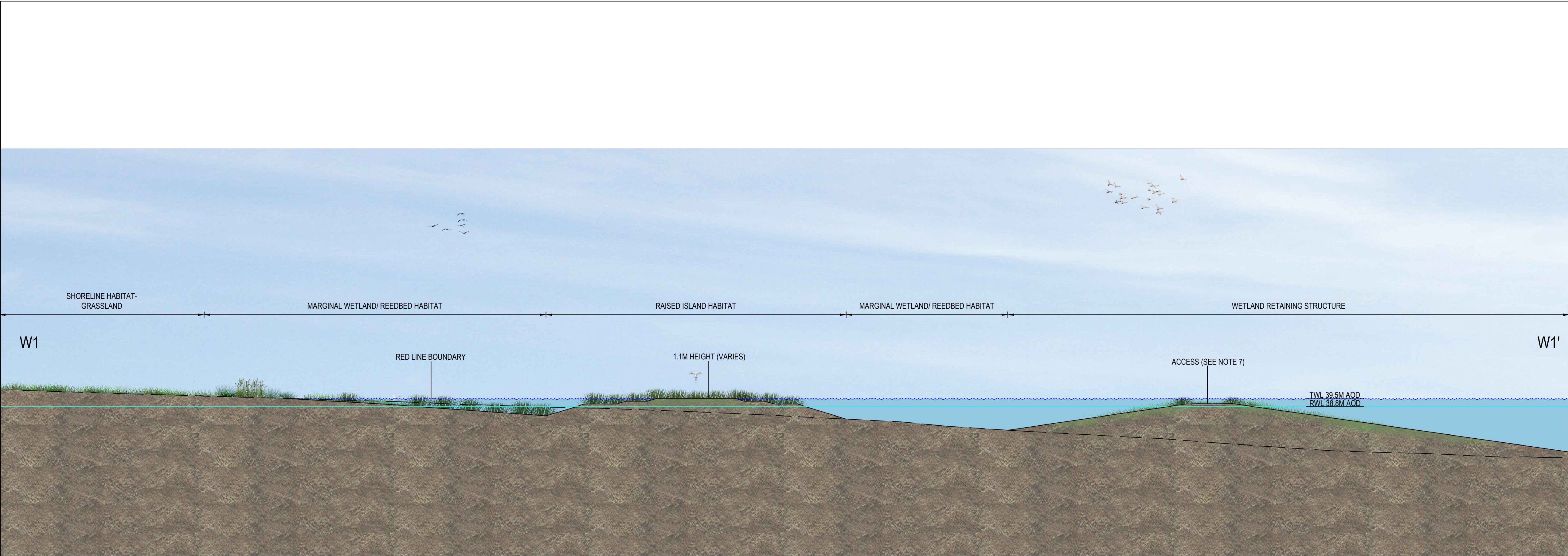
W1 - TYPICAL CROSS-SECTION THROUGH WETLAND ISLAND AND WETLAND RETAINING STRUCTURE SCALE 1:200
