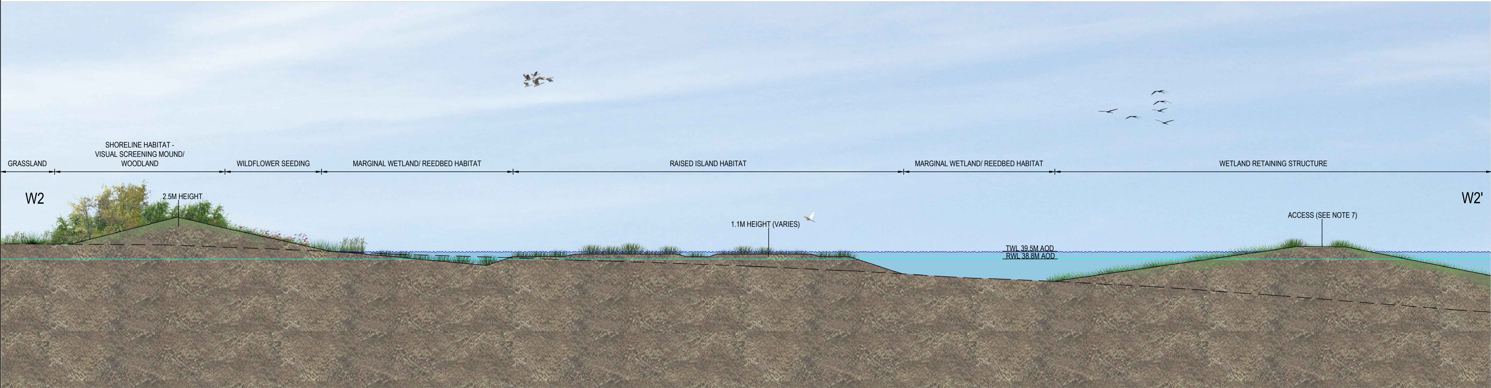
W2 - TYPICAL CROSS-SECTION THROUGH WETLAND ISLAND AND WETLAND RETAINING STRUCTURE SCALE 1:200
