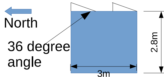
Front – road facing elevation
