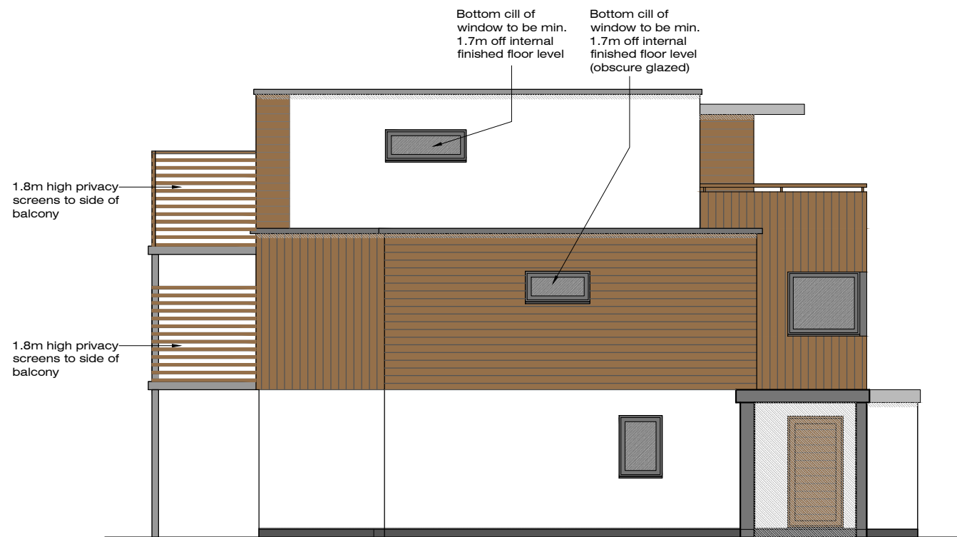
North (Side) Elevation - As Proposed
