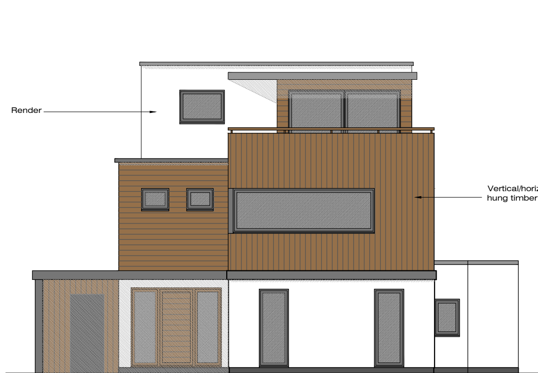
West (Front) Elevation - As Proposed
