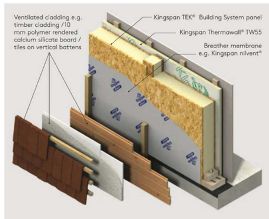
SIPs Panel Wall Section
