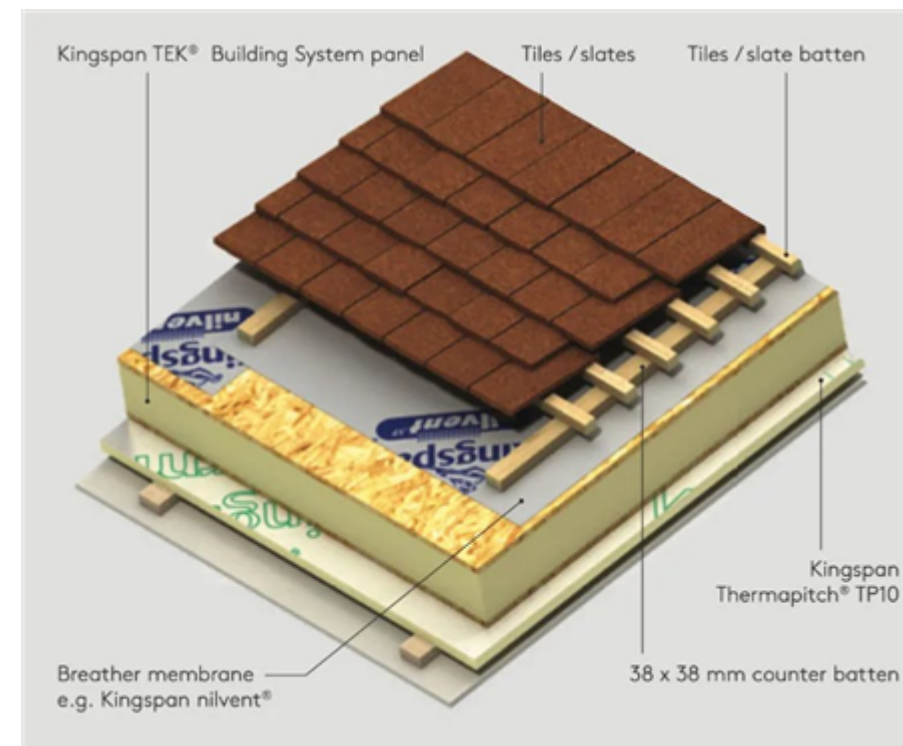
SIPs Panel Roof Section
