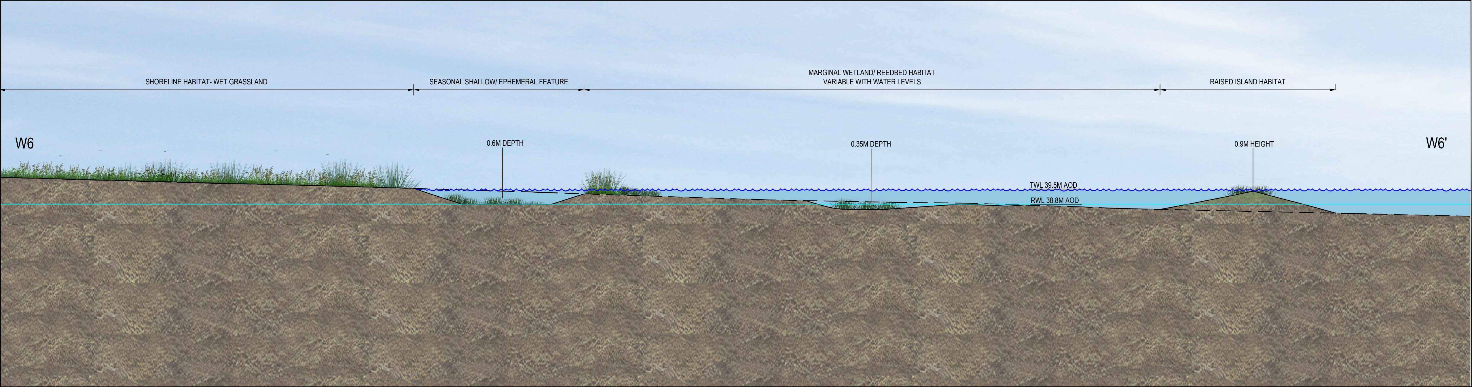
W6 - TYPICAL CROSS-SECTION THROUGH RAISED ISLANDS AND EPHEMERAL FEATURES SCALE 1:100
