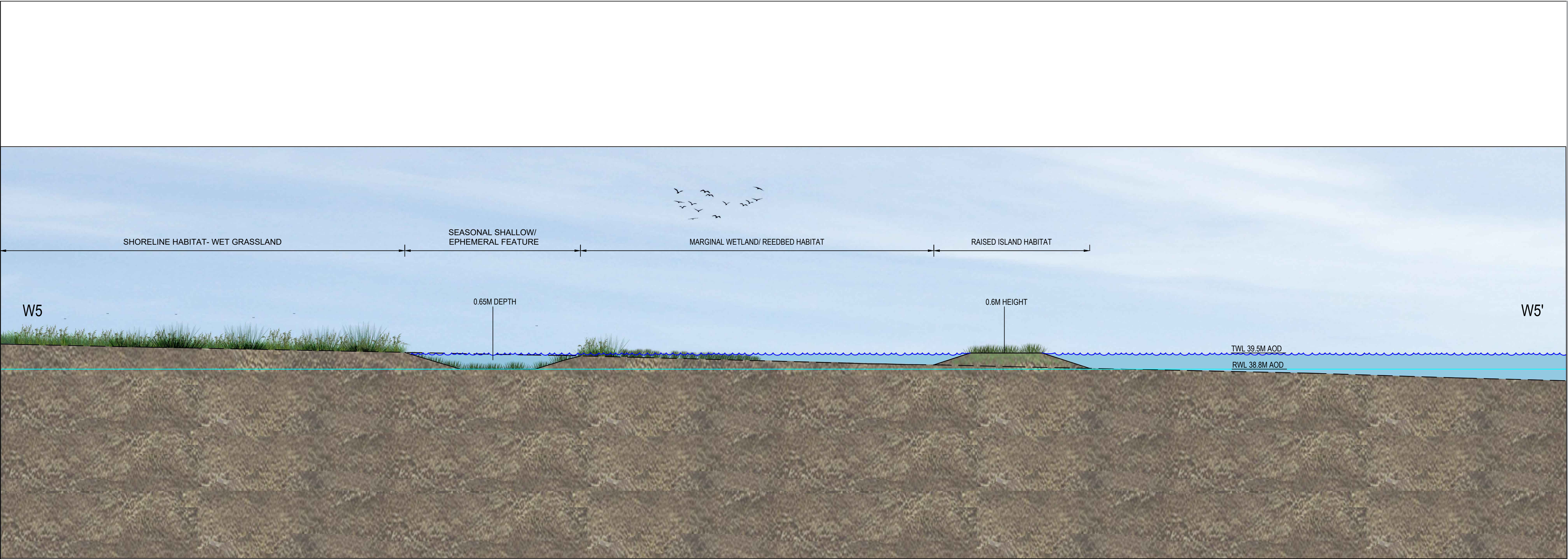
W5 - TYPICAL CROSS-SECTION THROUGH RAISED ISLANDS AND EPHEMERAL FEATURES SCALE 1:100
