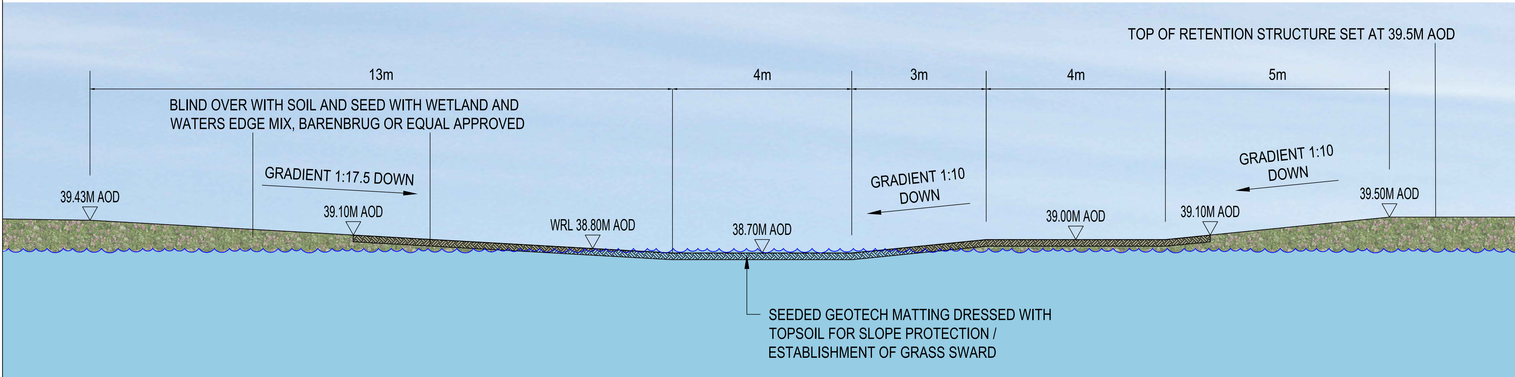
ELEVATION OF SPILLWAY FEATURE BETWEEN COMPARTMENTS 2 & 3 (WETLAND AREA) 1:50
