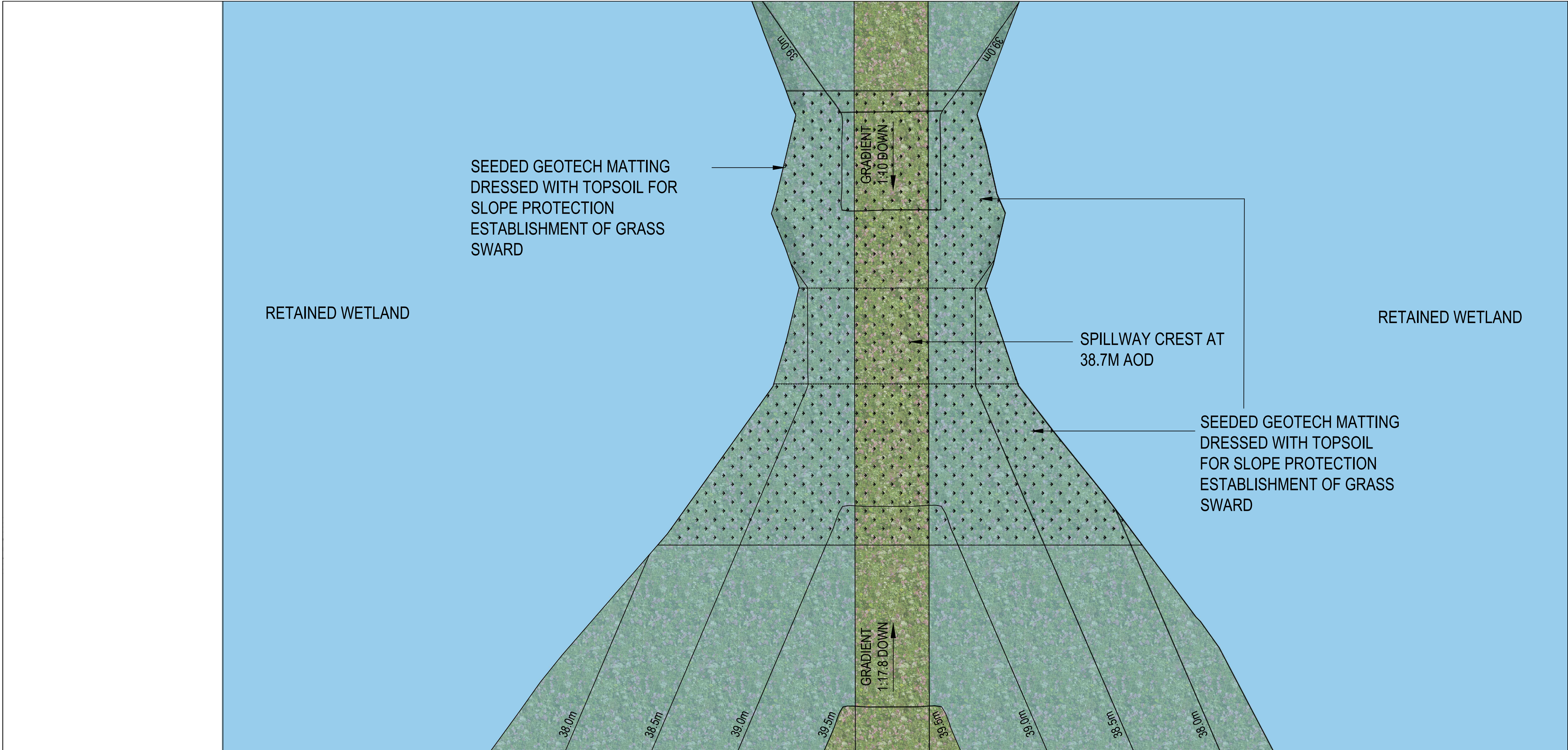
SPILLWAY FEATURE ALONG WETLAND RETAINING STRUCTURE (PLAN VIEW) 1:100
