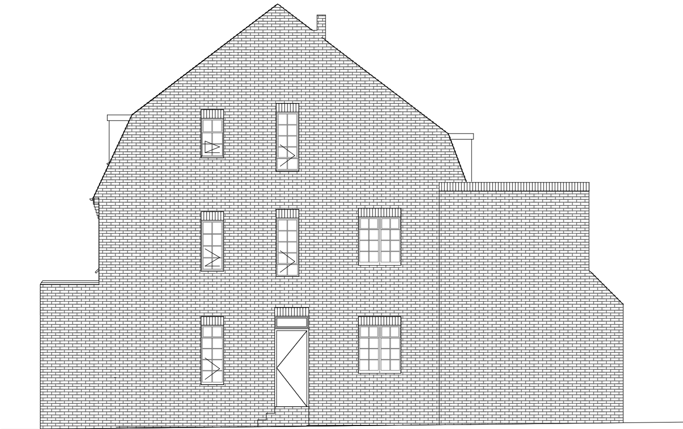
WEST ELEVATION 1:100
