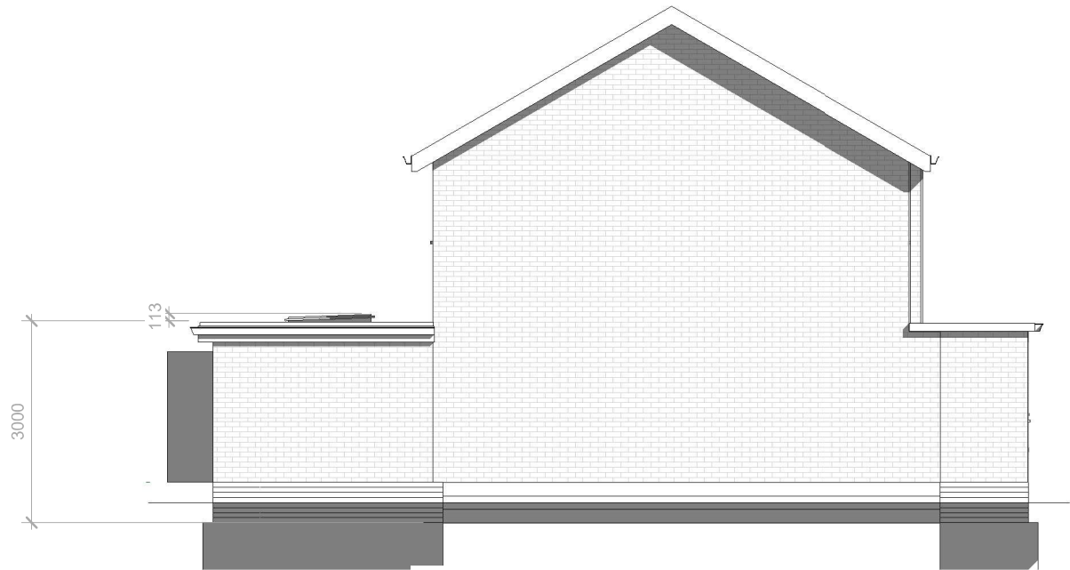
Proposed Elevation - Right
