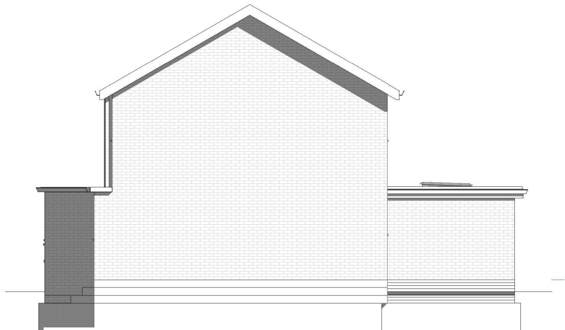
Proposed Elevation - Left
