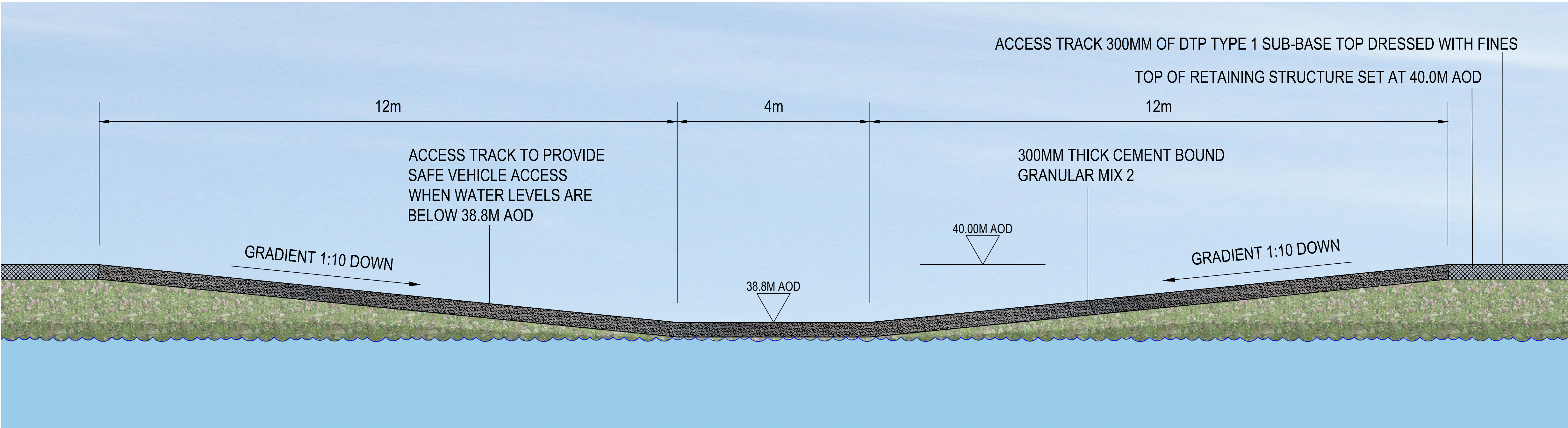
ELEVATION OF SPILLWAY FEATURE (WETLAND AREA) 1:50
