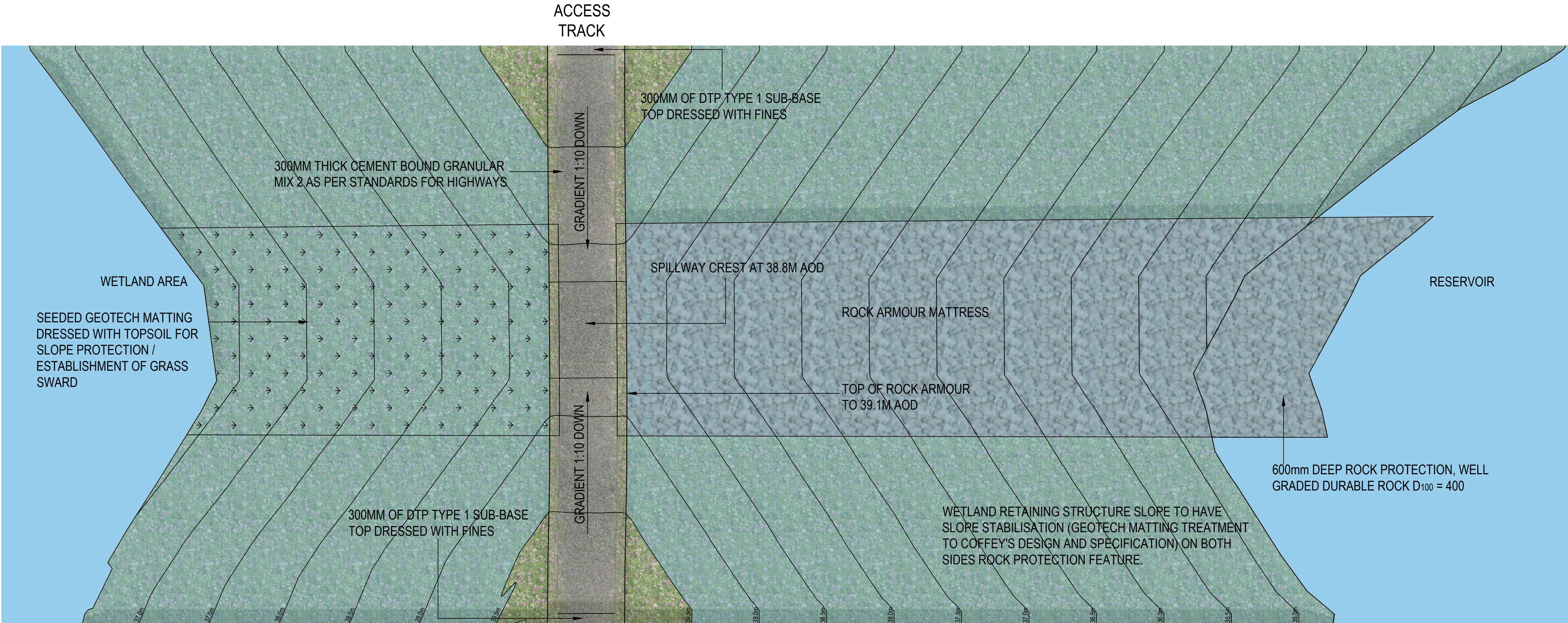
SPILLWAY FEATURE ALONG WETLAND RETAINING STRUCTURE (PLAN VIEW) 1:125
