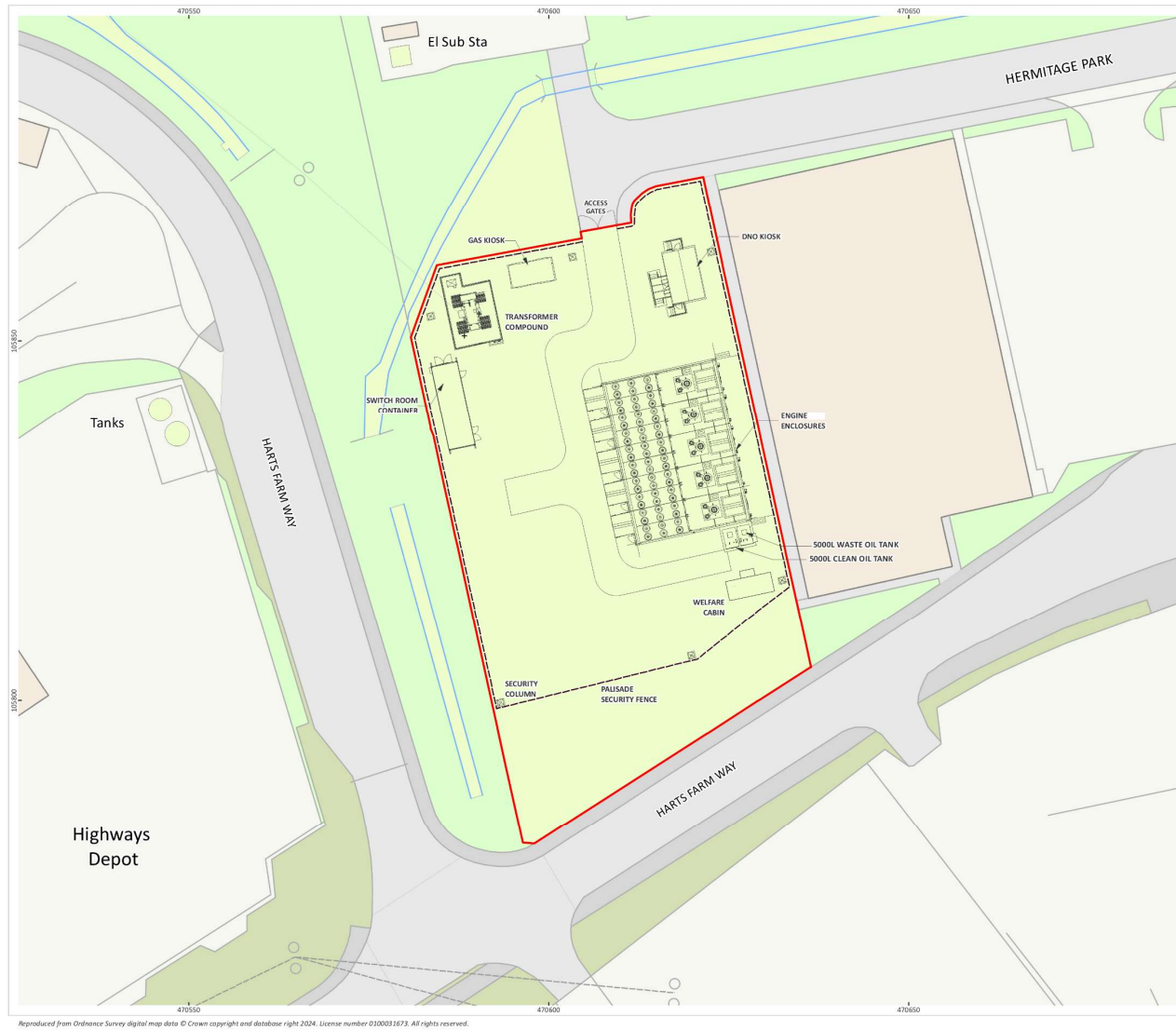
Figure 2.2 – Proposed site plan
