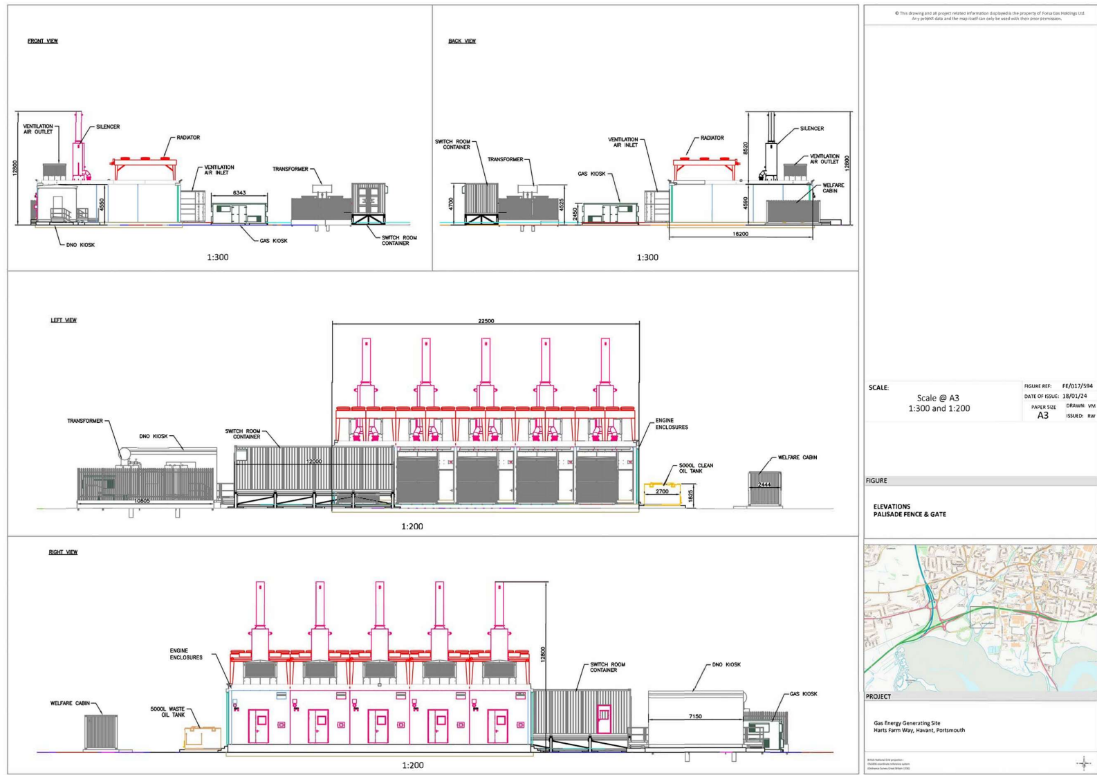
Figure 2.3 – Proposed elevations
