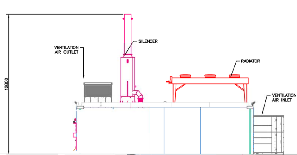
FRONT VIEW
