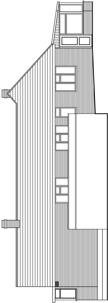
EXISTING NORTH ELEVATION
