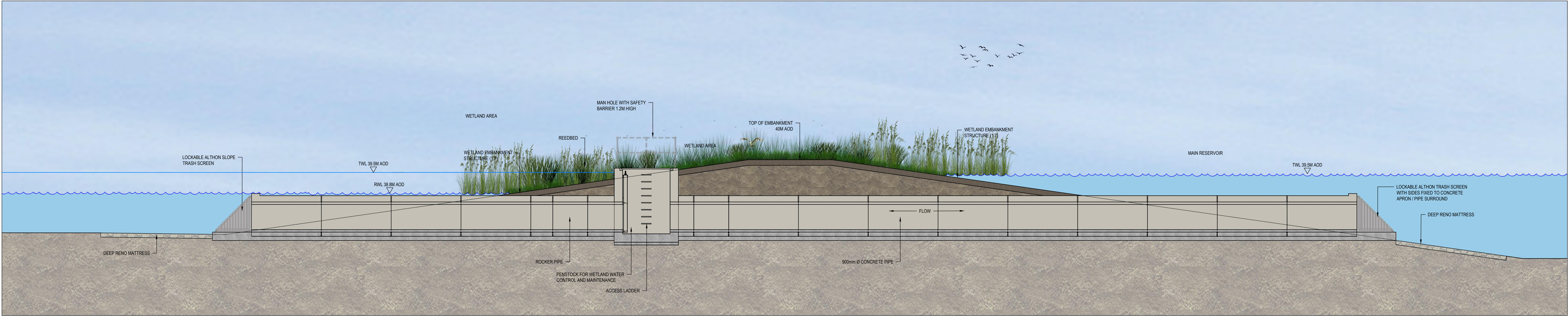
ELEVATION OF PENSTOCK CHAMBERS AND WETLAND RETAINING STRUCTURE
