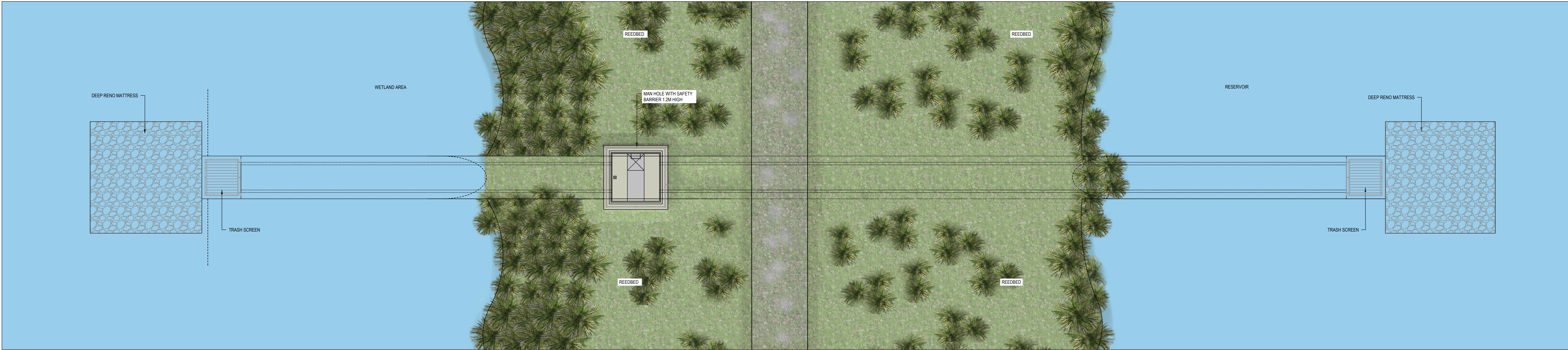
PENSTOCK CHAMBERS AND WETLAND RETAINING STRUCTURE (PLAN VIEW)
