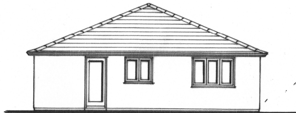
east elevation
