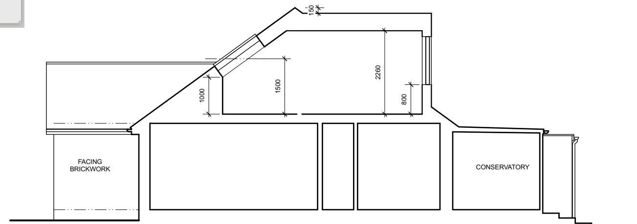
4 Proposed North Elevation Scale: 1:100
