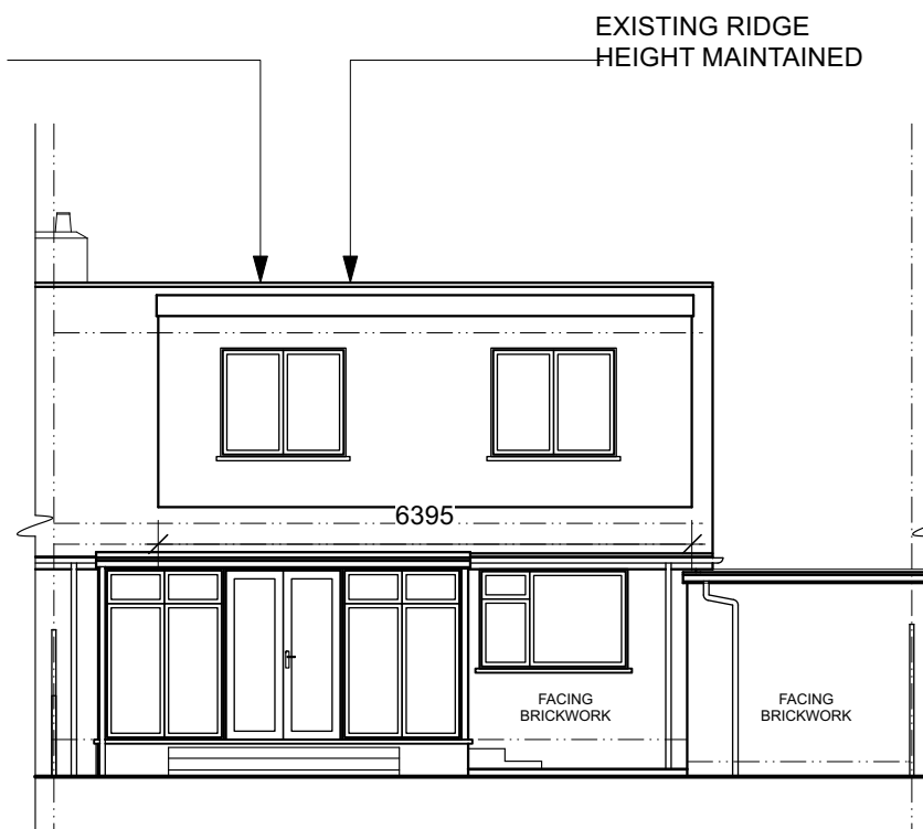
2 Proposed West Elevation Scale: 1:100
