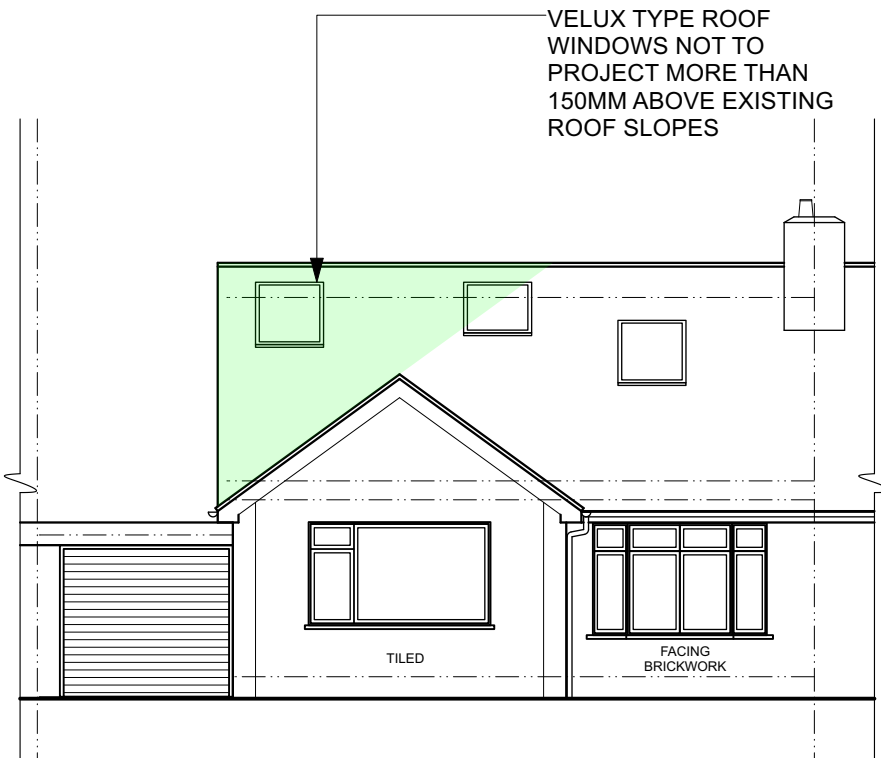
1 Proposed East Elevation Scale: 1:100
