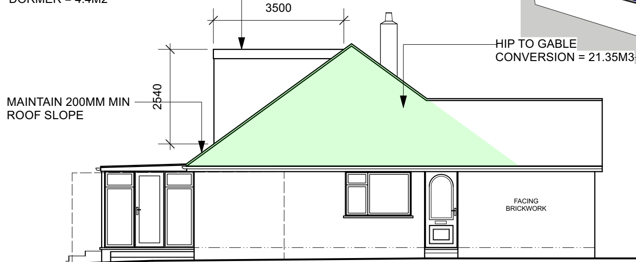
3 Proposed South Elevation Scale: 1:100
