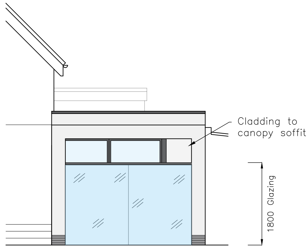
North Elevation
