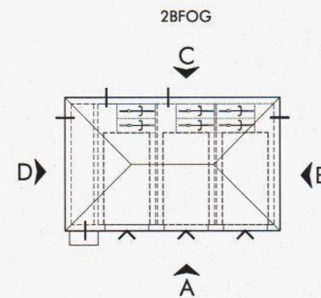
ROOF PLAN 1:200
