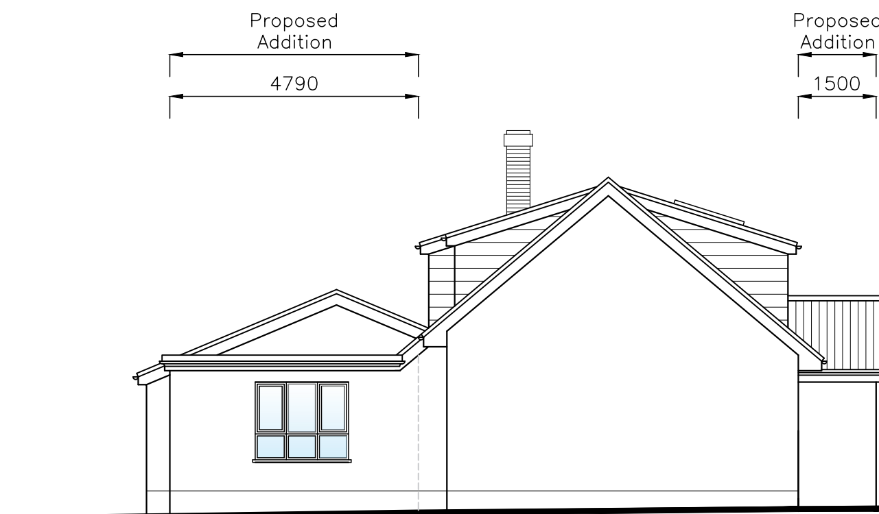
West Elevation
