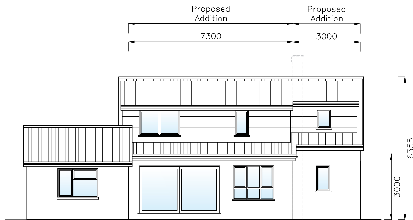
South Elevation
