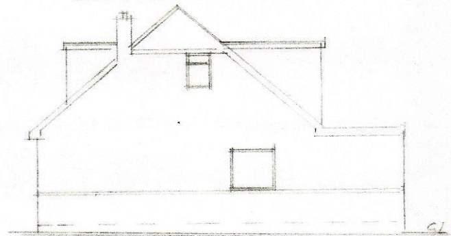
EXG. REAR ELEV. 1:100
