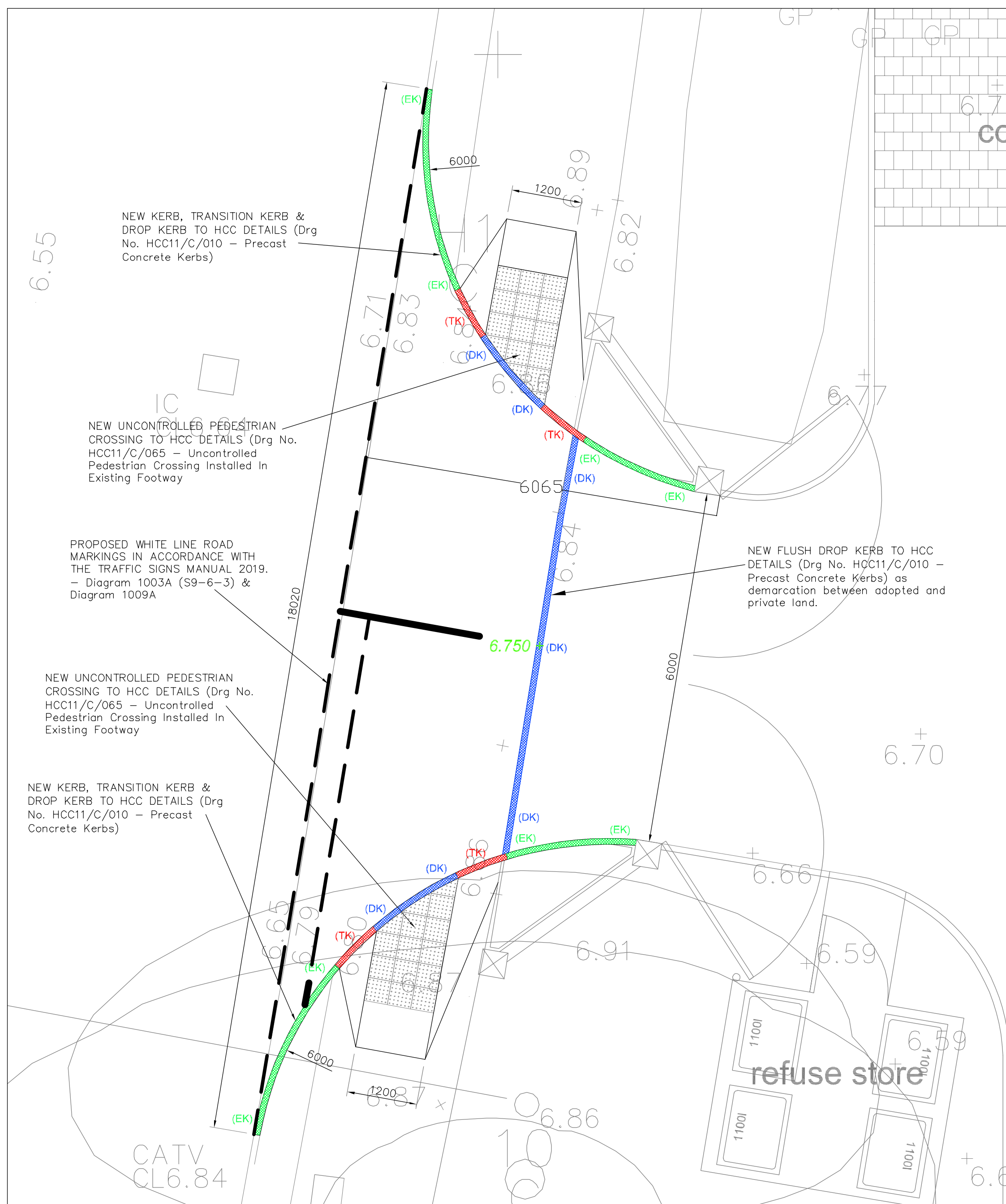
PROPOSED ENTRANCE PLAN SHOWING PROPOSED LAYOUT AND KERB LINES 1:50
