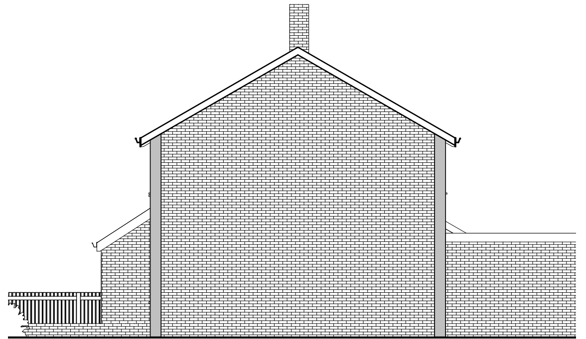
2 North Elevation 1 : 100
