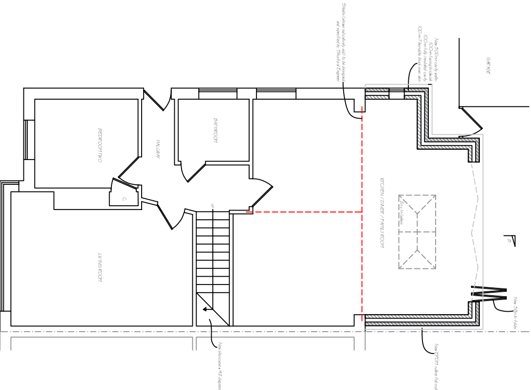
Proposed Ground Floor Plan 1:100 @ A3
