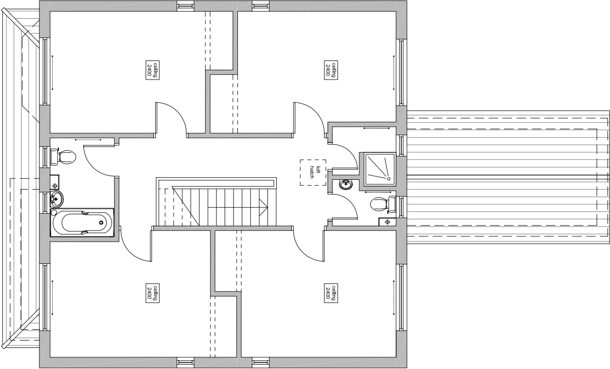
existing 1st floor plan
