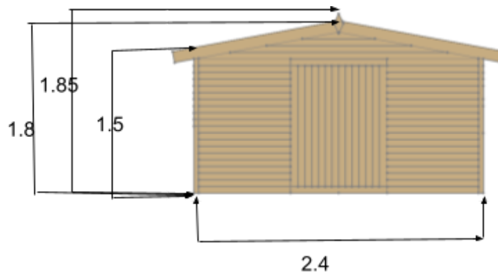
Front(East side)
