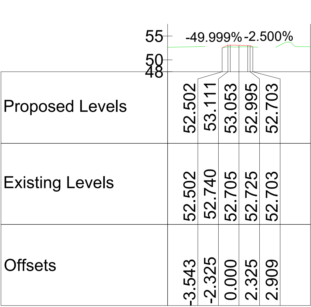
Chainage 1060.000
