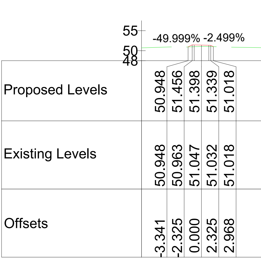
Chainage 1160.000
