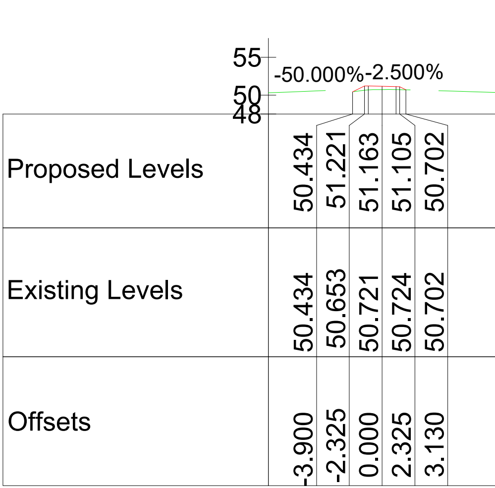
Chainage 1180.000
