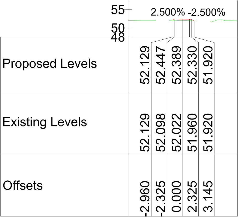
Chainage 1080.000
