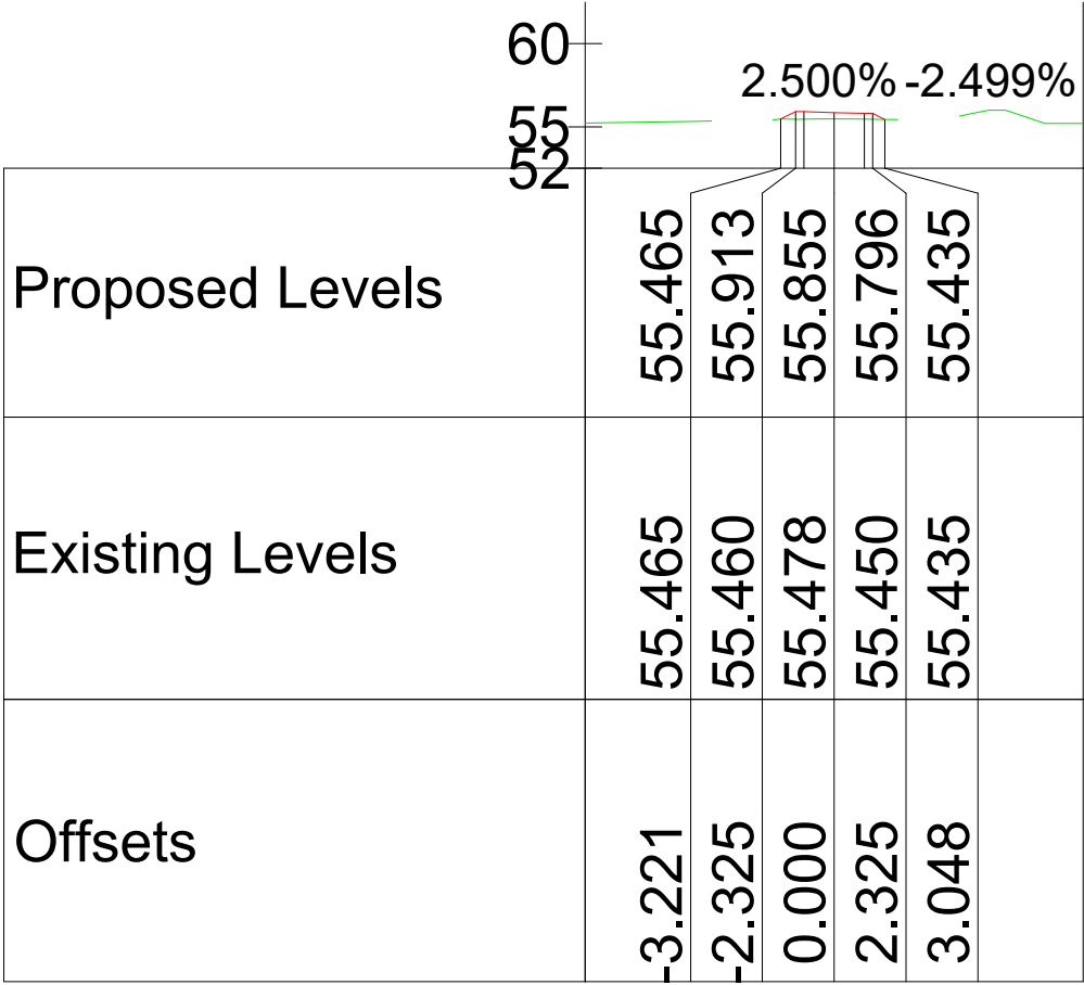
Chainage 960.000
