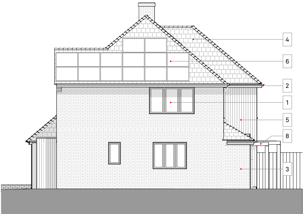
1:100 South Elevation - Proposed
