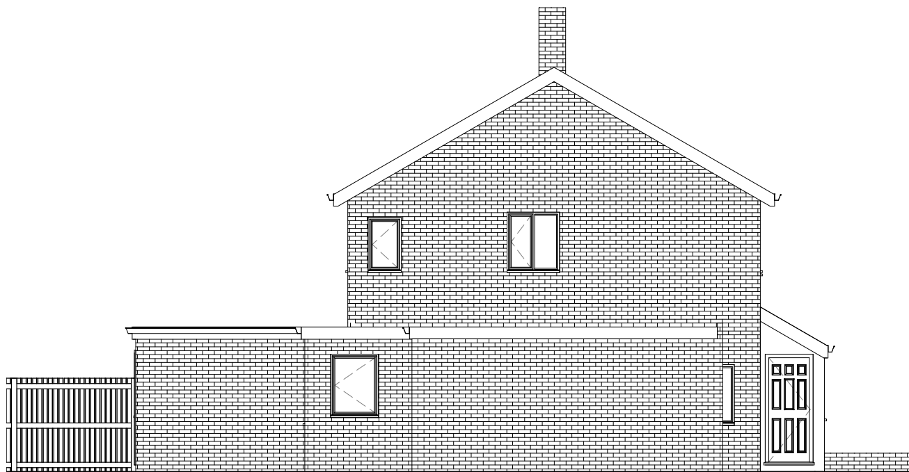
3 South Elevation 1 : 100
