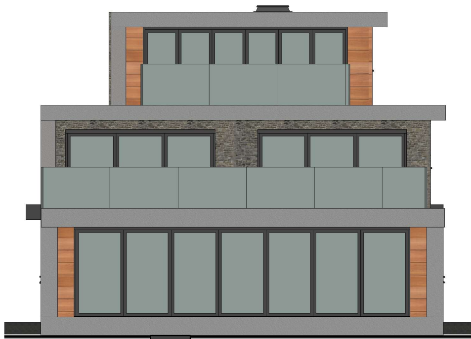
3 South Elevation 1 : 100
