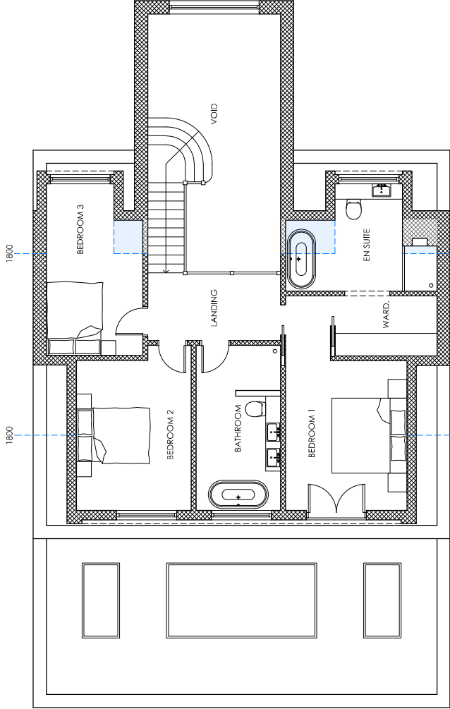
PROPOSED LOFT PLAN
