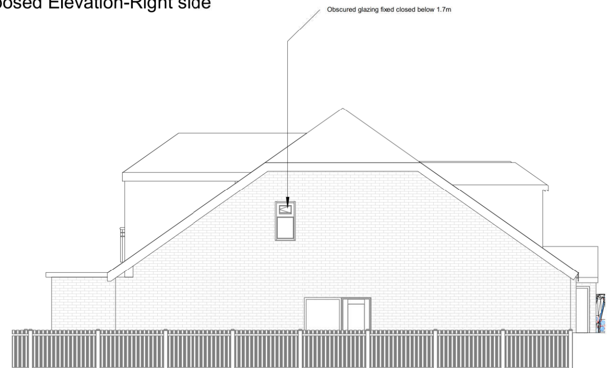
Proposed Elevation-Right side
