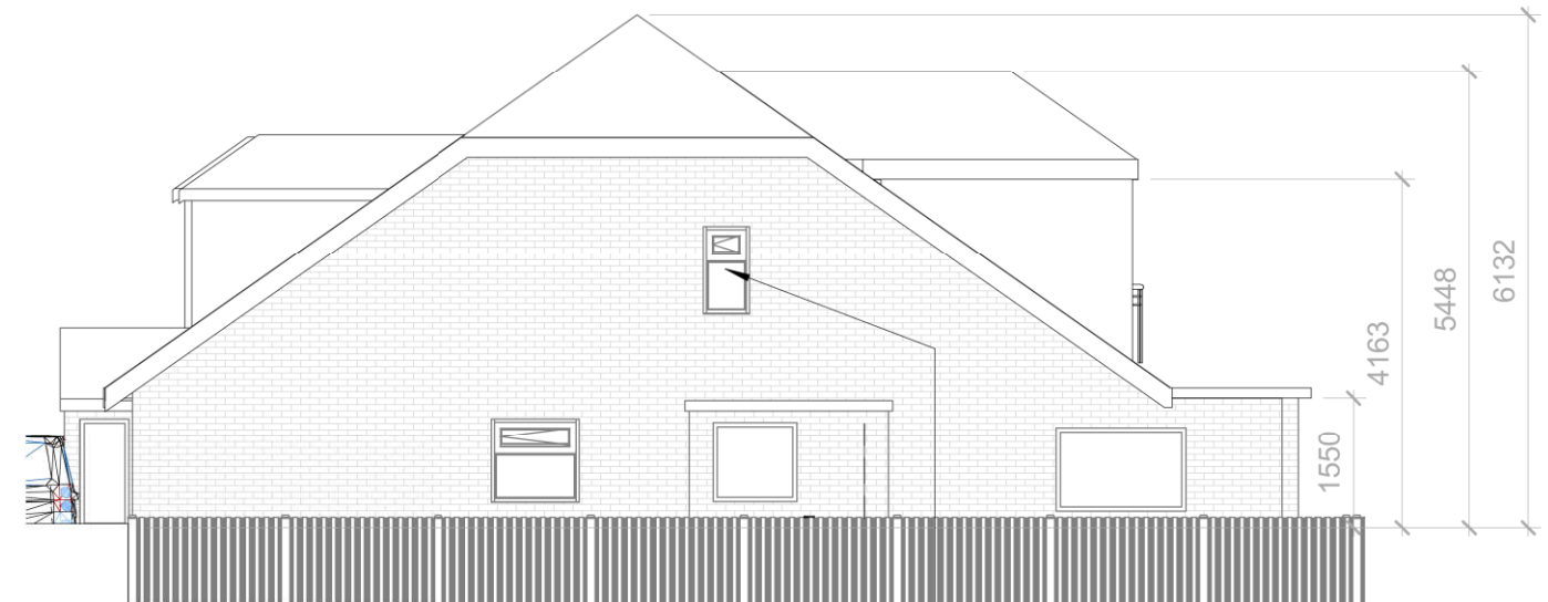
Proposed Elevation-Right side
