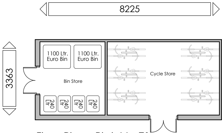
Floor Plan - Plot 66 - 71 Plot 152 - 157
