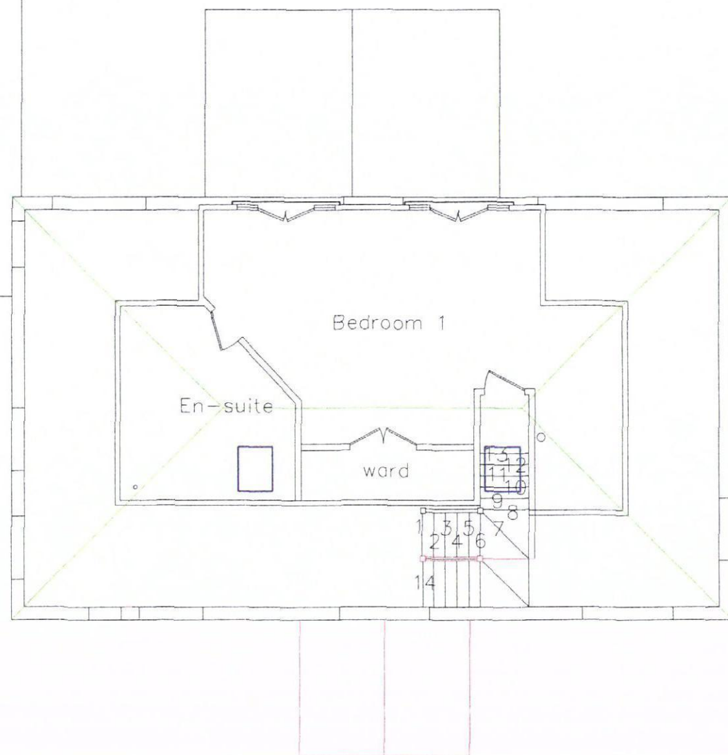
EXISTING LOFT FLOOR
