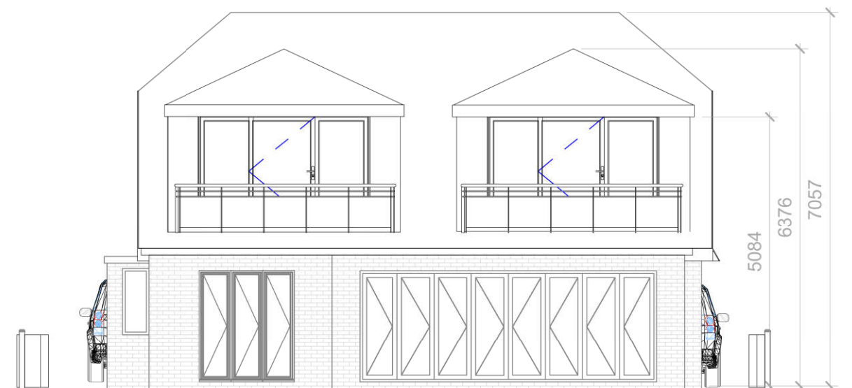
Proposed Elevation-Rear
