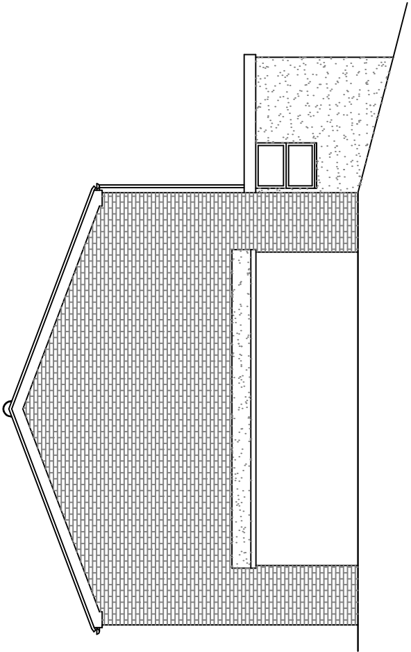
EXISTING SIDE ELEVATION (with shed)
