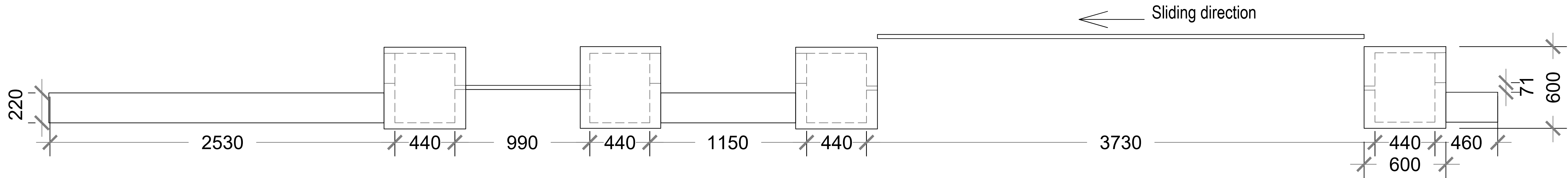
Proposed Gate Plan Scale 1:20
