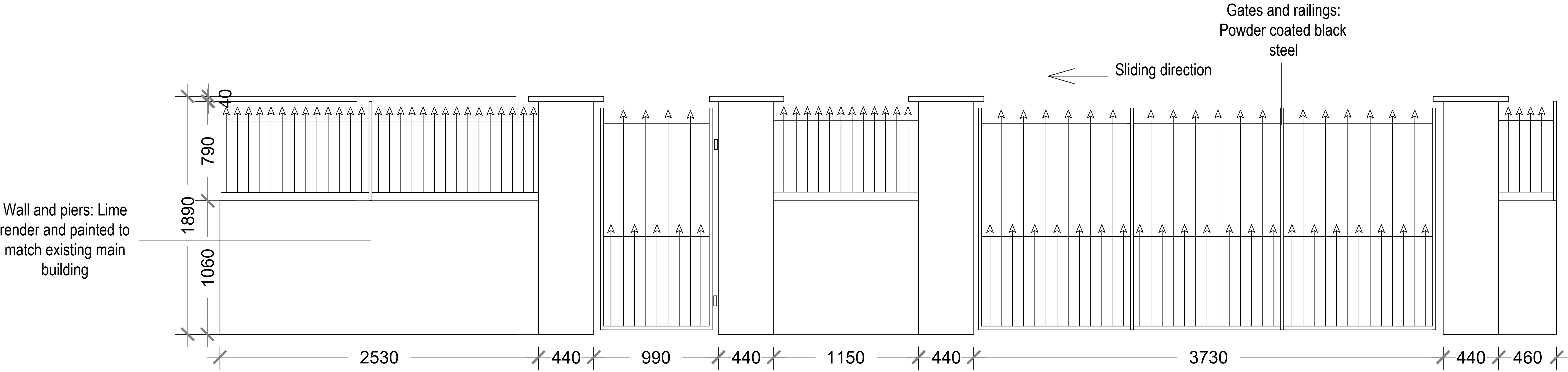
Proposed Front Gate Elevation Scale 1:20
