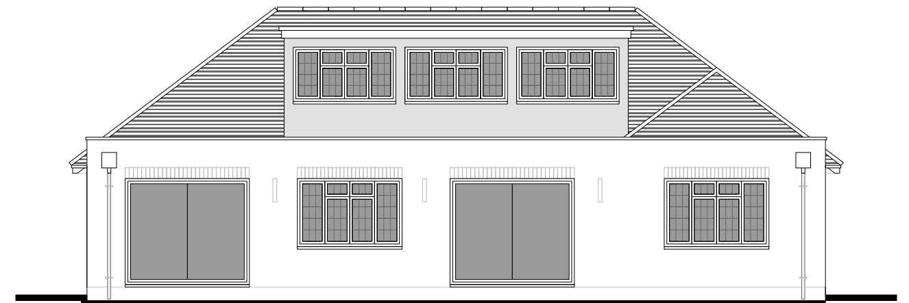
Proposed Rear Elevation at 1:100 scale SOUTH EAST
